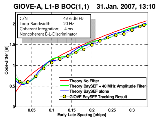
Figure 6 Examples for measured code-jitter in dependency of early-late-spacing of GIOVE L1-B together with theoretical expectations.
